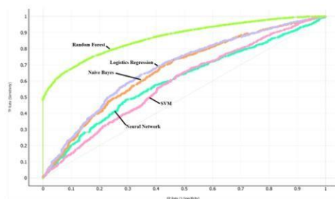
Figure 6: ROC curve of five predictive models
