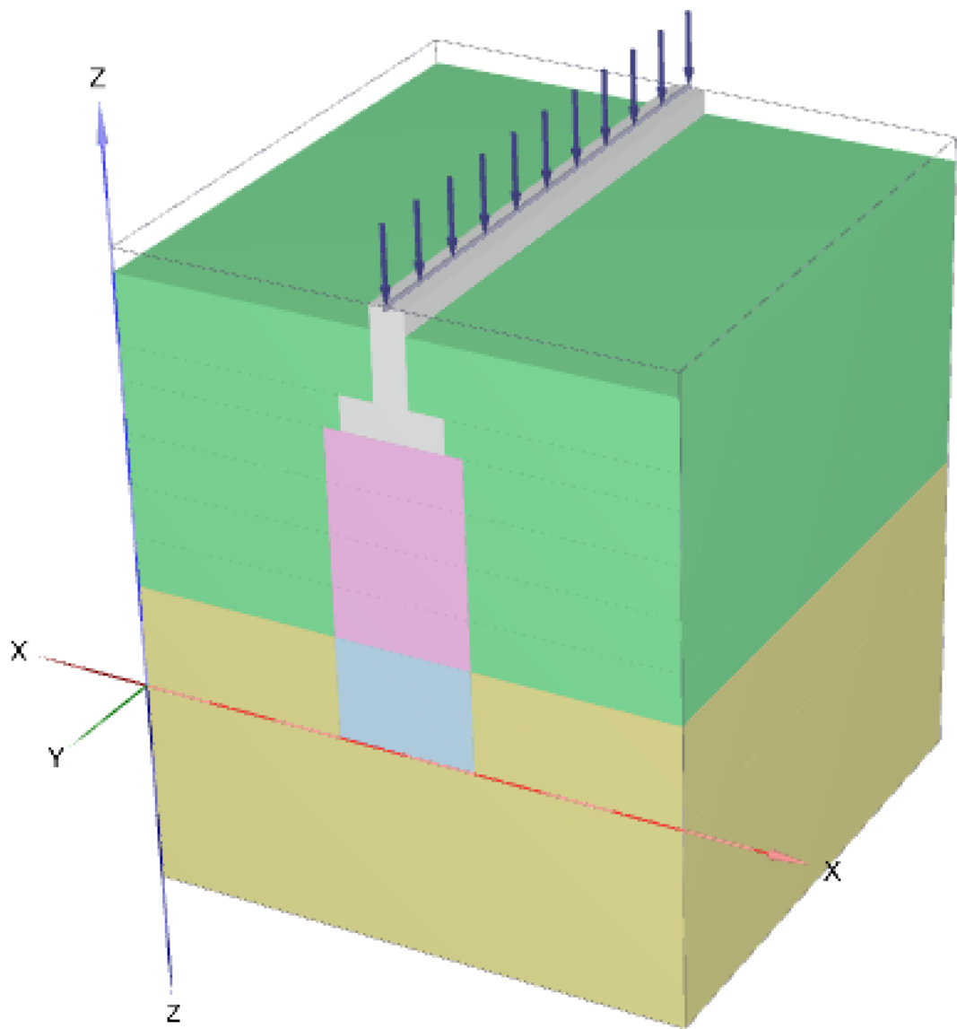
Figure 5. PLAXIS FE model
