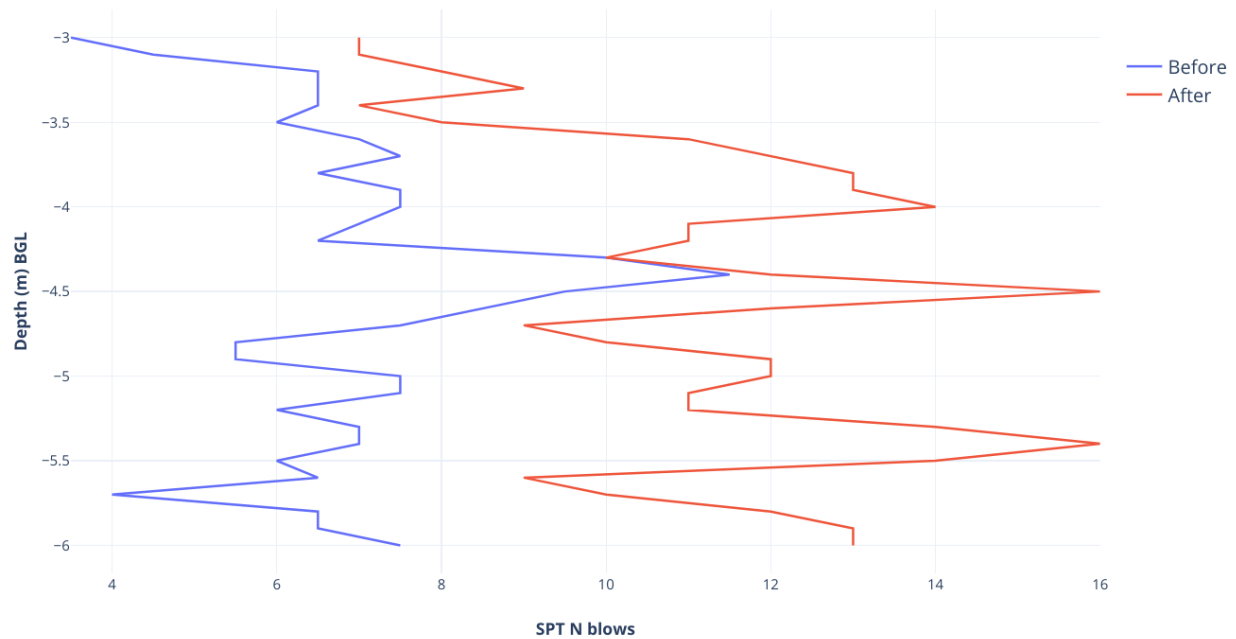
Figure 4. SPT blow count before and after injection
