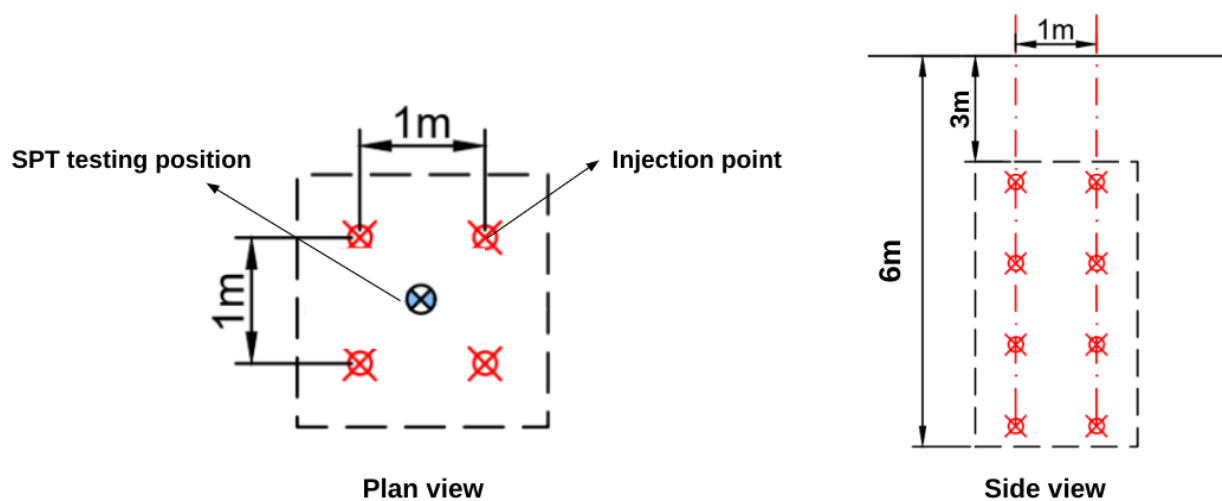
Figure 3. Test Injection layout
