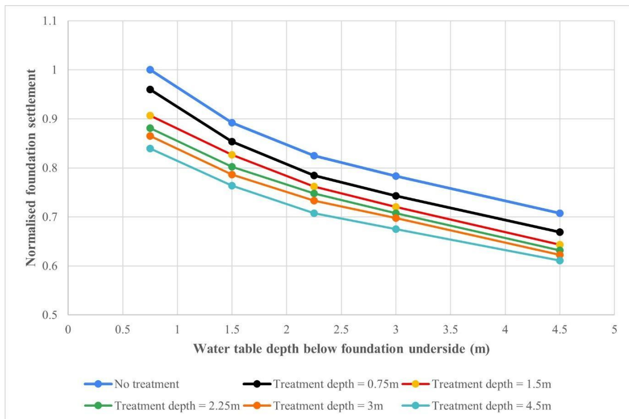
Figure 6. Foundation settlement as a result of different water table levels and treatment depths
