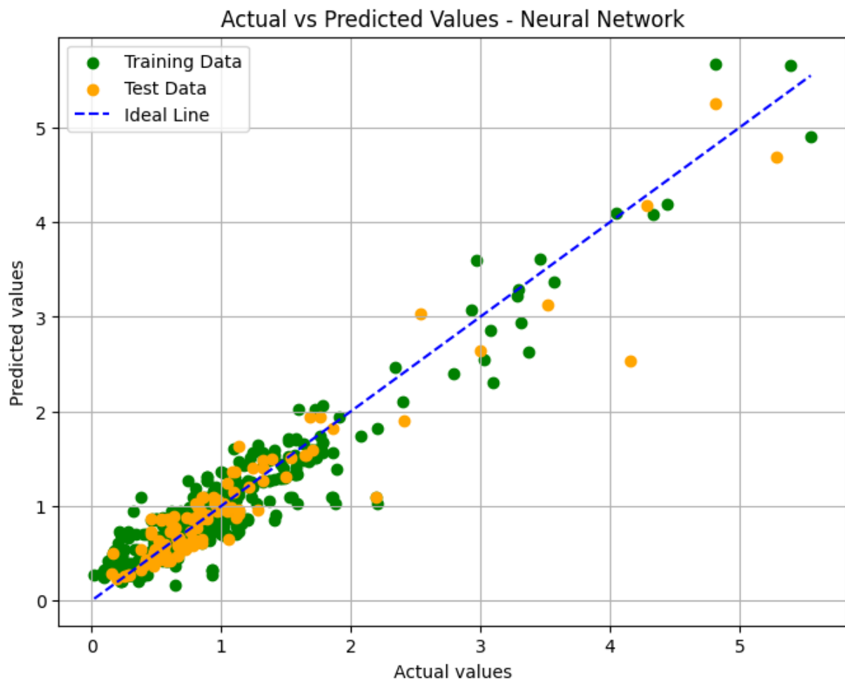
Figure 4. Predicted vs. Actual T-period for ANN Model
