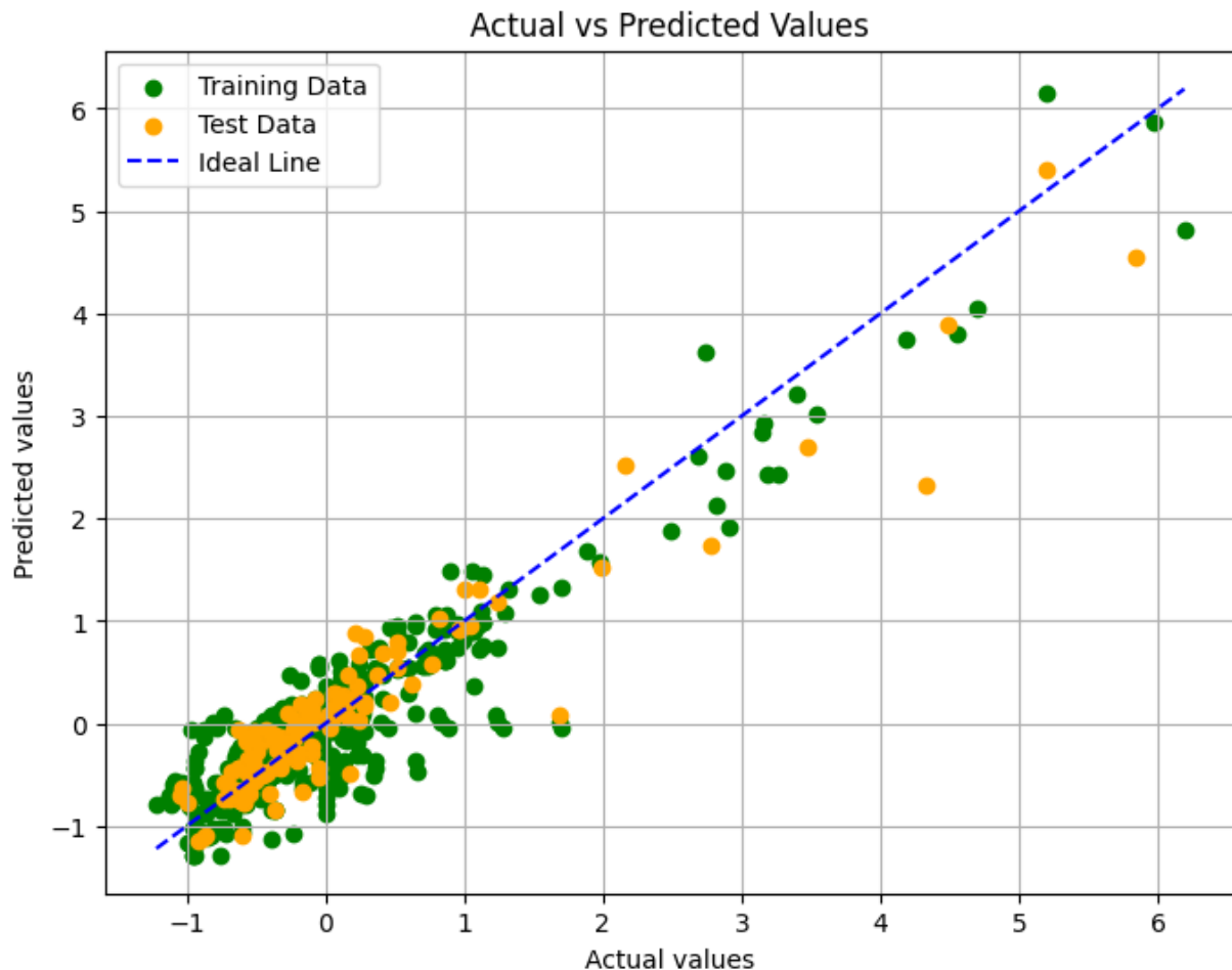
Figure 9. Predicted vs. Actual T-period for Linear Regression Model
