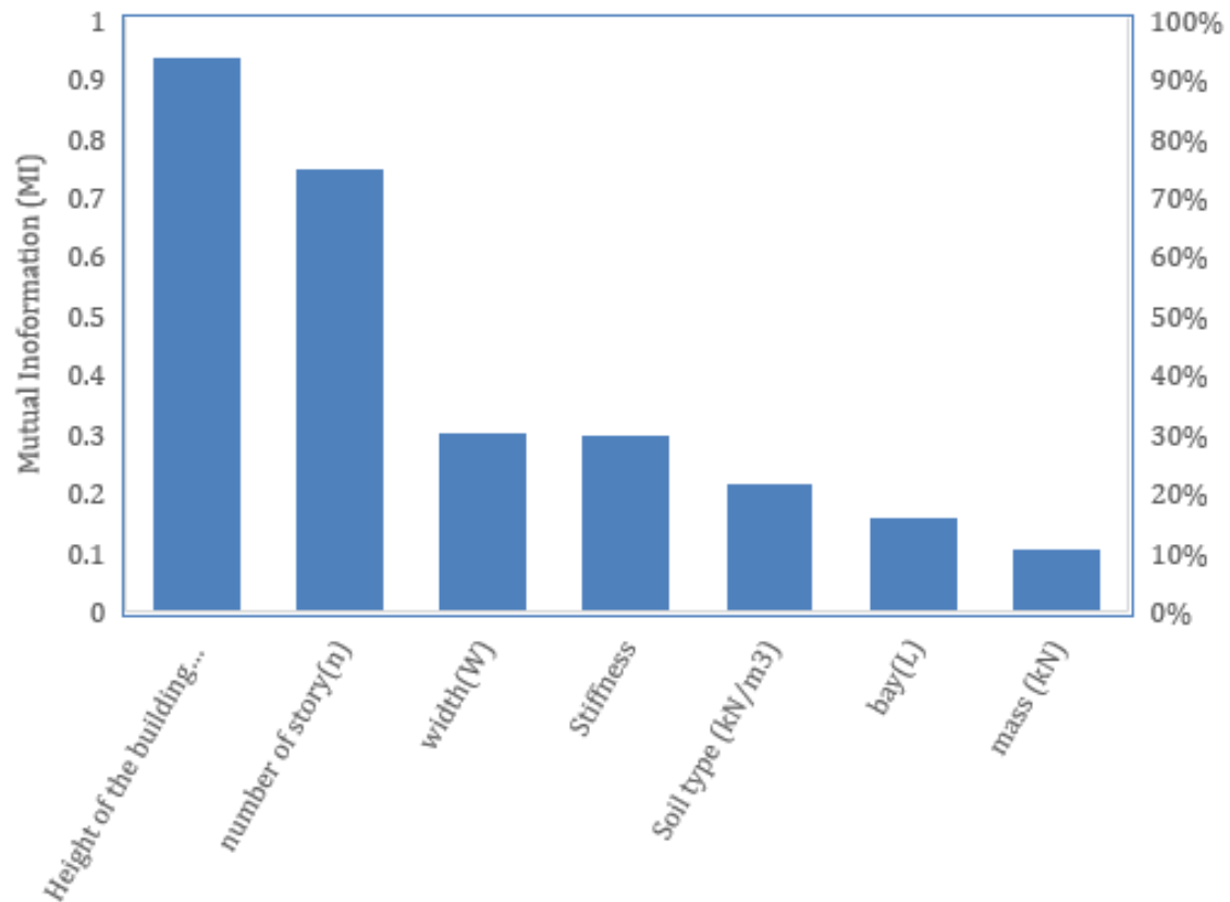
Figure 2. Mutual dependencies of the selecting of the data set prior to learning
