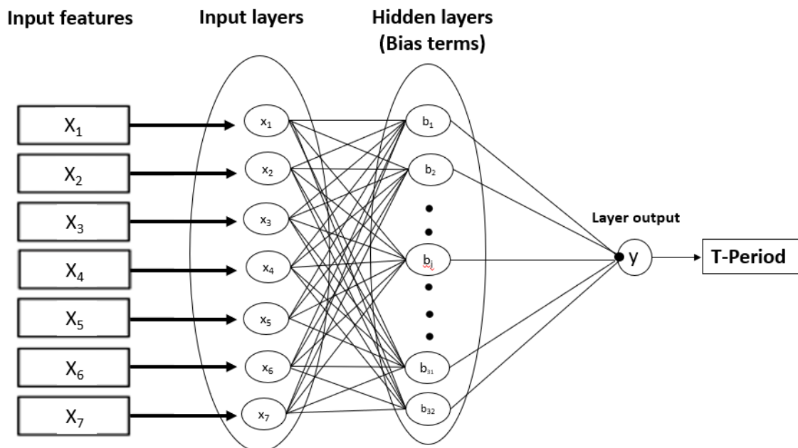
Figure2. Schematic for architecture of BPA based neuron network carried out in this work. [28]
