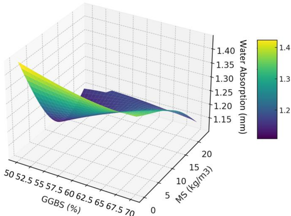
Fig. 4. 3D Surface-Plot between MS, GGBS and Water Absorption
