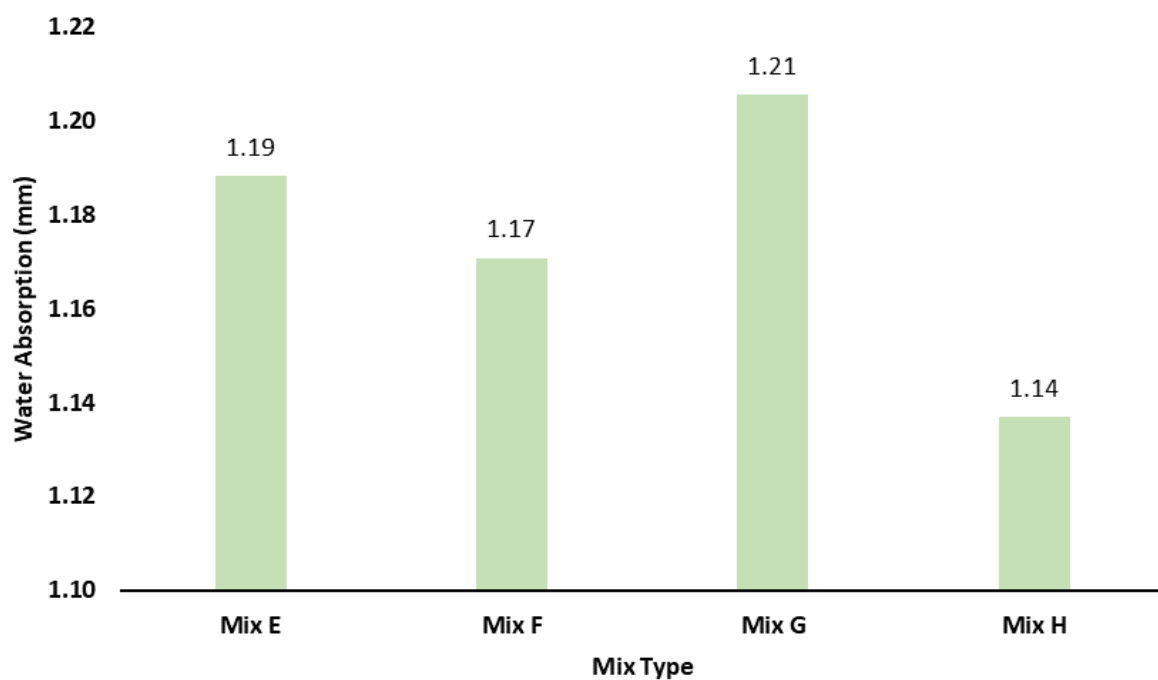
Fig. 3. Water Absorption for C40/20 Concrete Mixes with Varying Micro silica Content
