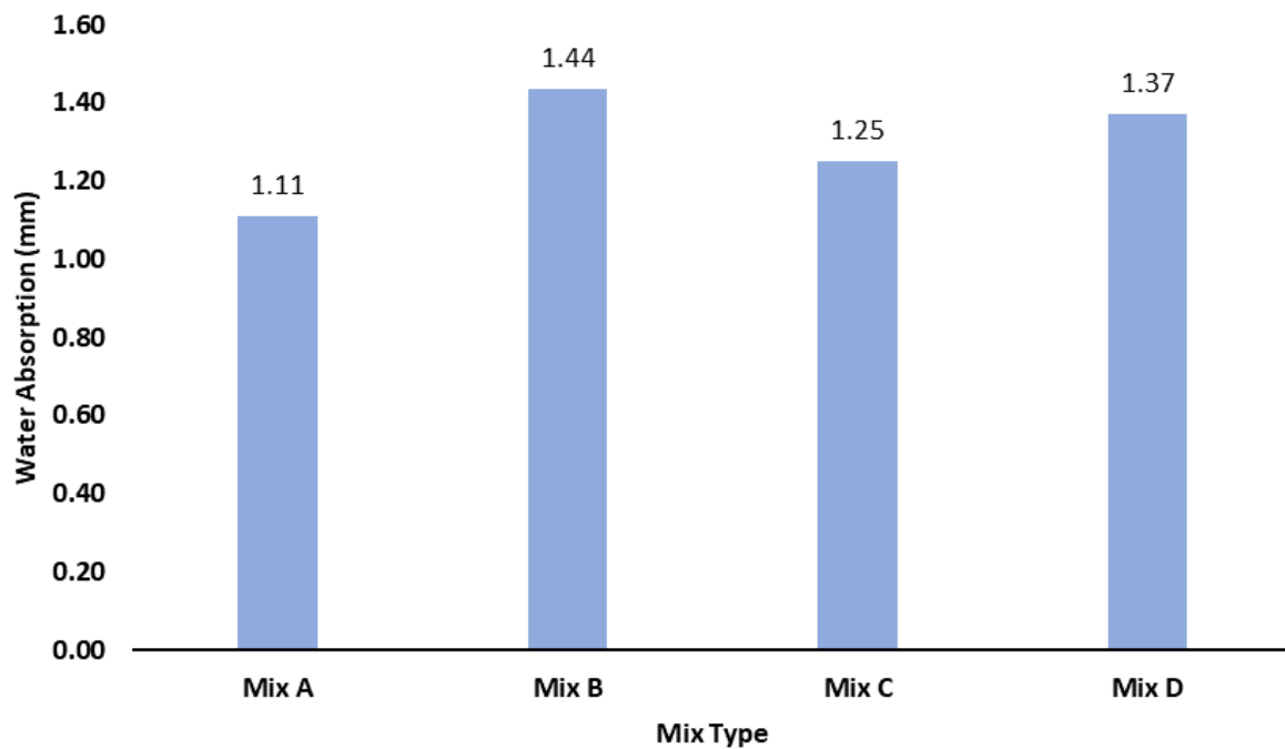
Fig. 2. Water Absorption for C40/20 Concrete Mixes with Varying Micro silica Content
