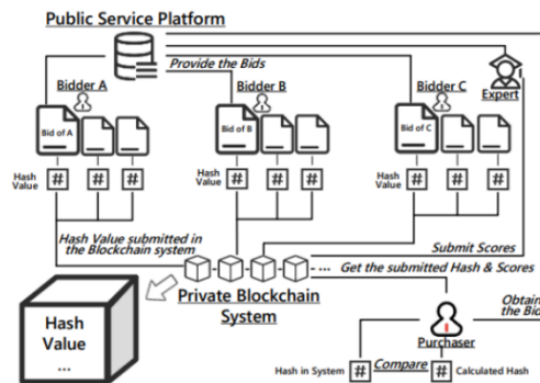
Figure 3. Blockchain-Based E-Tendering System of Tendering Evaluation
