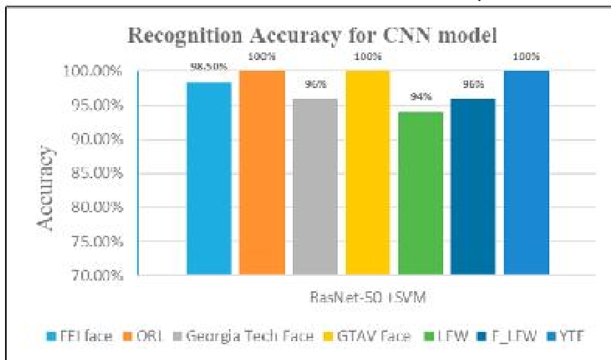
Fig 2.3 Shows the Accuracy of the ResNet-50 +SVM model on facial recognition databases[1].
