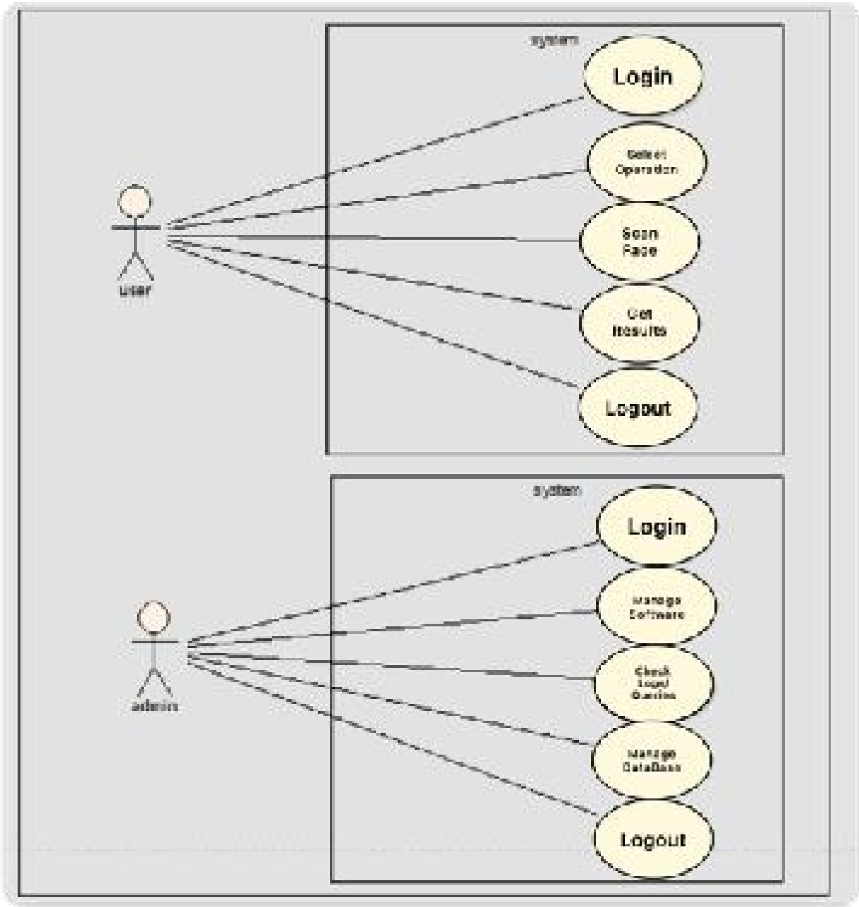
Figure 3. 1 Shows the use case diagram for the proposed system. 3.10 Flow Chart Diagram:
