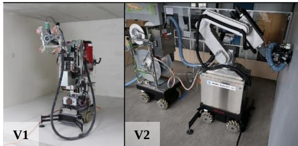
Figure 2: Developed Robots
