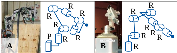
Figure 5: Developed Manipulators
