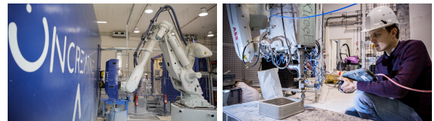
(a) Concreateive: industrial robotic 3DCP cell (b) ENPC: R&D robotic 3DCP cell
