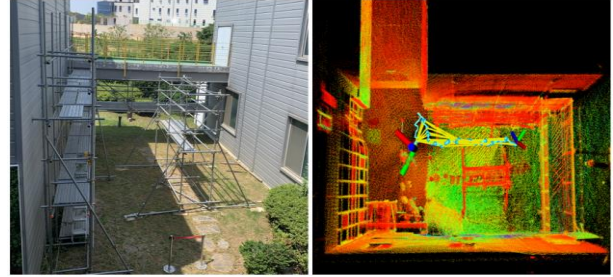
(a) (b) Figure 4. Site A dataset; (a) photograph of Site A, (b) registered point clouds
