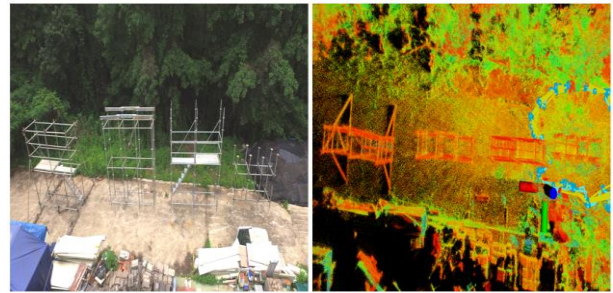
(a) (b) Figure 5. Site B dataset; (a) photograph of Site B, (b) registered point clouds
