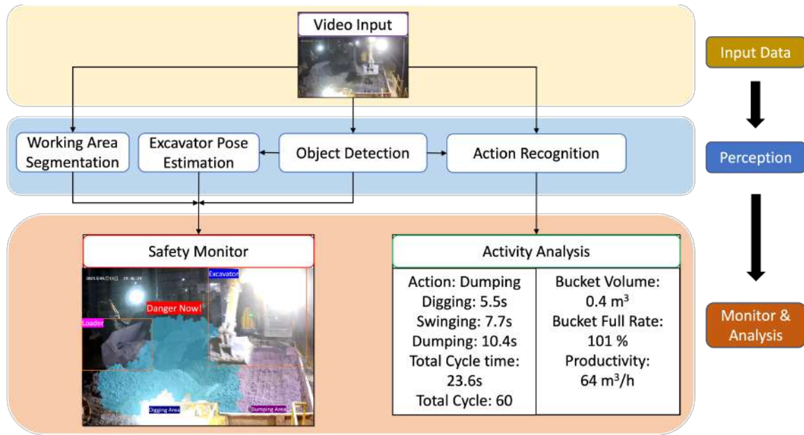
Figure 1. Autonomous Excavator System (AES) activity analysis and safety monitoring system pipeline.
