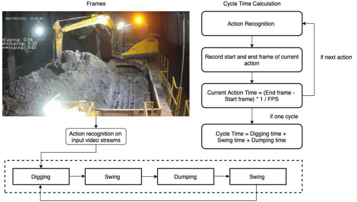
Figure 5. Excavator working cycle.
