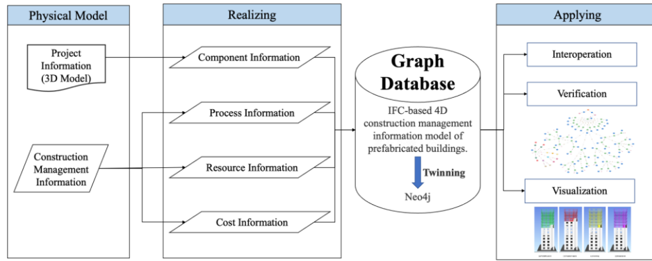
Fig.1 Proposed Framework
