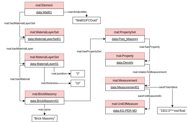
Figure 3. Example of use of the materials ontology
