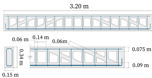
Figure 2. Design of the second prototype. The rebars are represented in blue.
